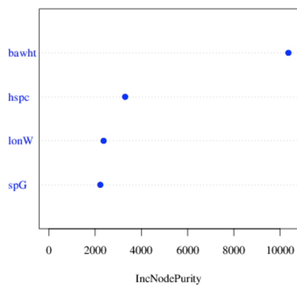
C MZ 47 – FIA Biomass Variable Importance
