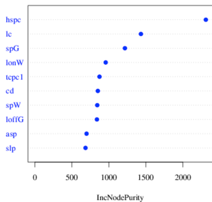
B MZ 47 – NCE Biomass Variable Importance
