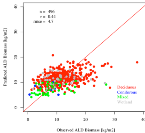
F MZ 47 – FIA Biomass Bootstrap Validation
