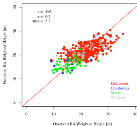
E MZ 47 – NCE Biomass Bootstrap Validation
