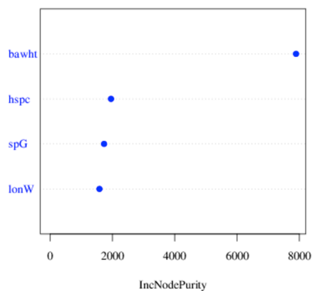
C MZ 47 – FIA Biomass Variable Importance
