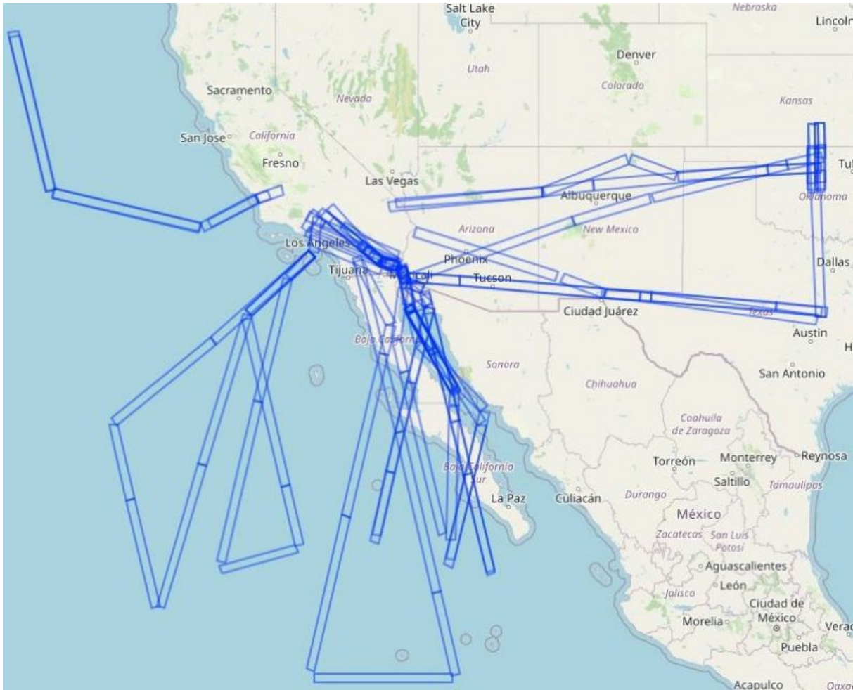
Figure 2. Flight tracks in this dataset represented as rectangular polygons. Basemap: © OpenStreetMap contributors.
