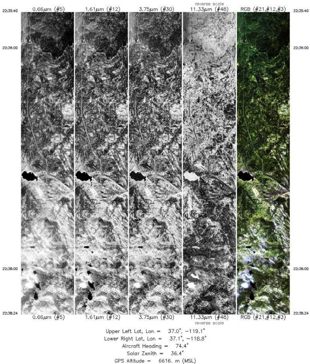
Figure 1. Single band images and an RGB composite image from flight track 6 acquired on 19 June 2013 over the Sierra National Forest east of Fresno, California, U.S. Source: MASTERL1B_1300406_06_20130619_2235_2238_V01.jpg
