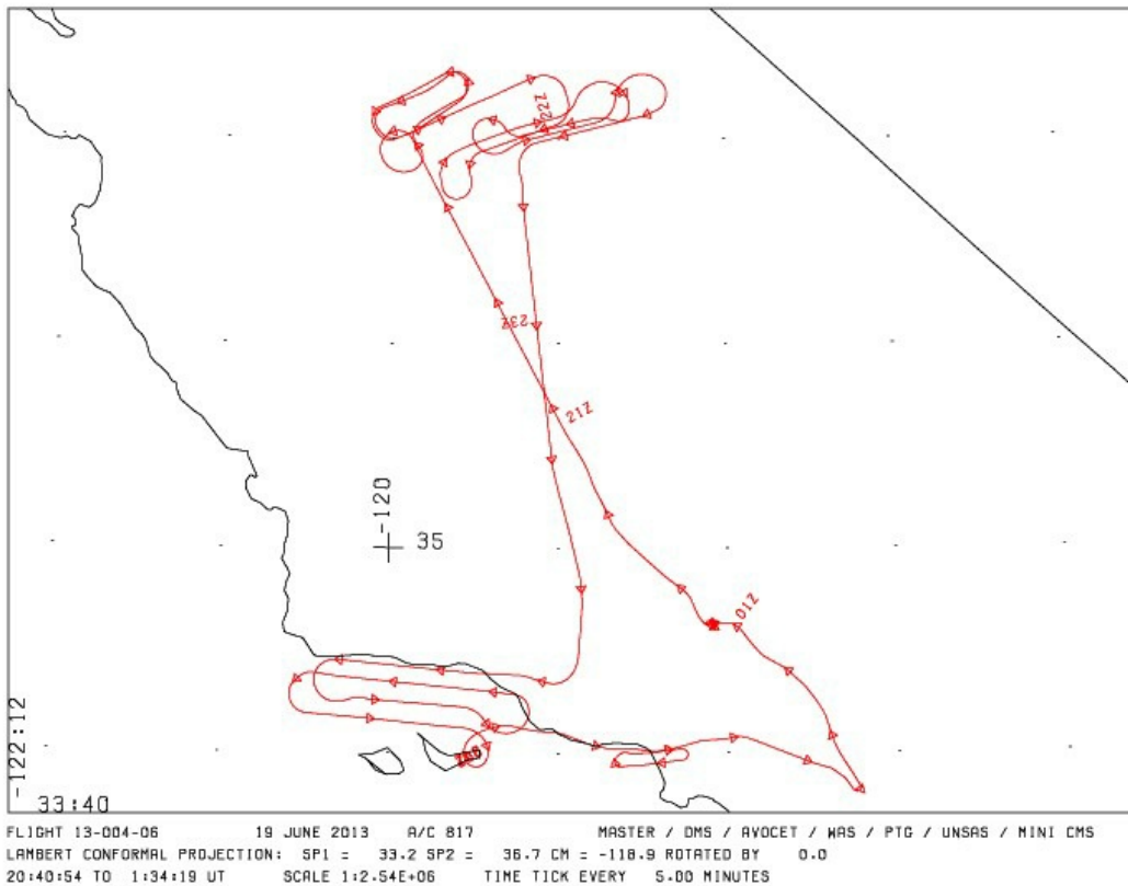
Figure 3. Flight path for Flight 1300406, flown on 19 June 2013. Flight 1300406 and 11 flight tracks occurred over southern California, U.S. Source: MASTER_1300406_20130619_flightpath.gif
