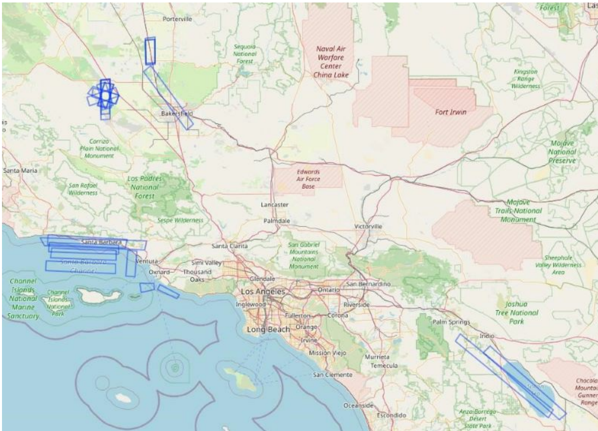
Figure 2. Flight tracks in this dataset represented as rectangular polygons. Map shows southern California, U.S. Basemap: © OpenStreetMap contributors.
