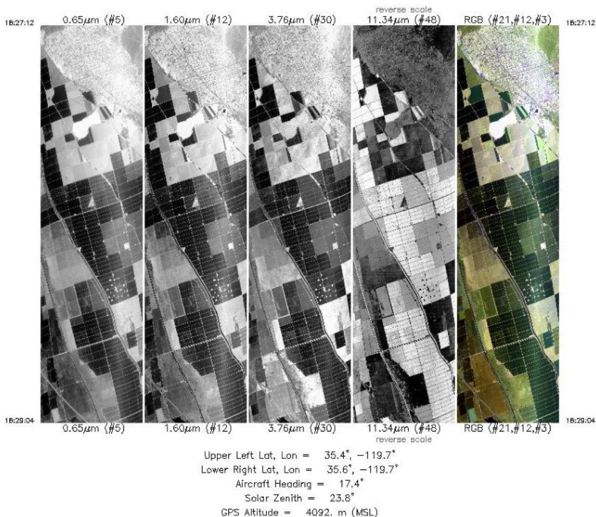
Figure 1. Single band images and an RGB composite image from flight track 6 acquired on 28 June 2011 over California's Central Valley WNW of Bakersfield, California, U.S. Source: MASTERL1B_1100303_03_20110628_1827_1829_V01.jpg
