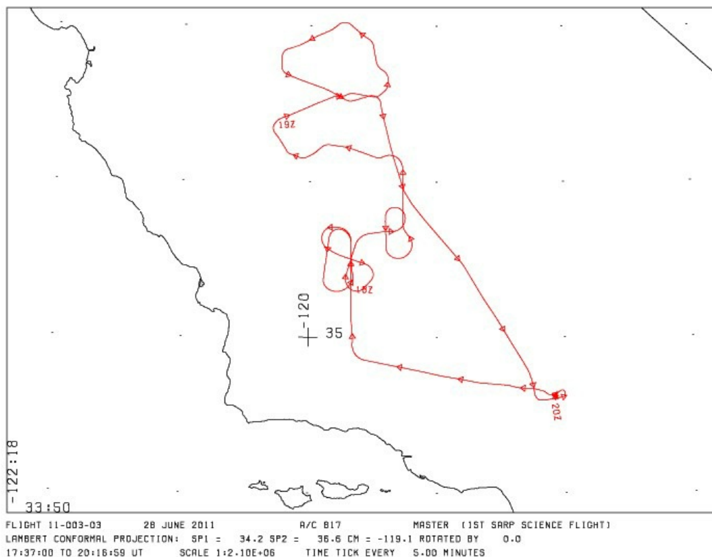
Figure 3. Flight path for Flight 1100303, flown on 28 June 2011. Flight 1100303 and 4 flight tracks occurred over southern California, U.S. Source: MASTER_1100303_20110628_flightpath.gif
