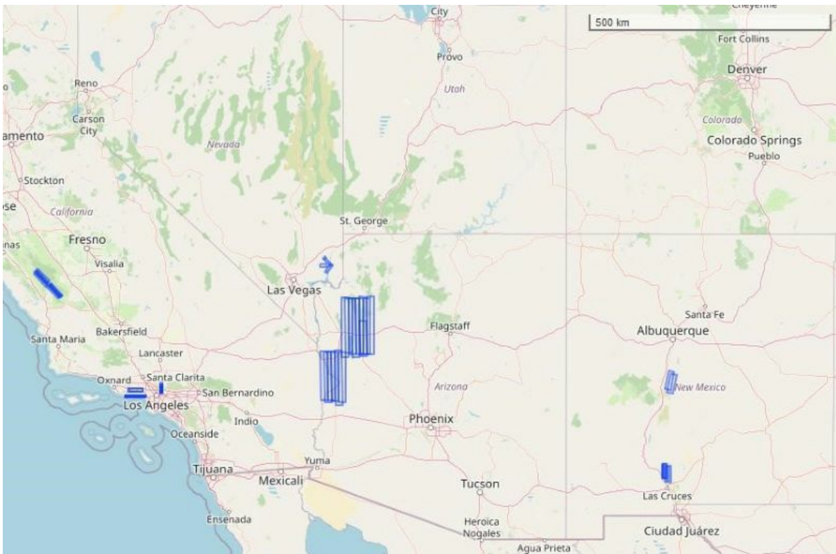
Figure 2. Flight tracks in this dataset represented as blue rectangular polygons. Map shows southwestern U.S. Basemap: © OpenStreetMap contributors.
