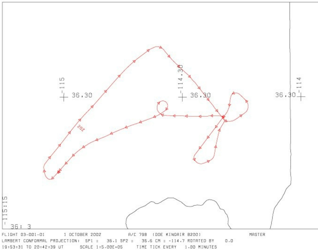
Figure 3. Flight path is shown for 01 October 2002. Flight 0300101 and 4 flight tracks over the vicinity of Lake Mead east of Las Vegas, Nevada. Source: MASTER_0300101_20021001_flightpath.gif
