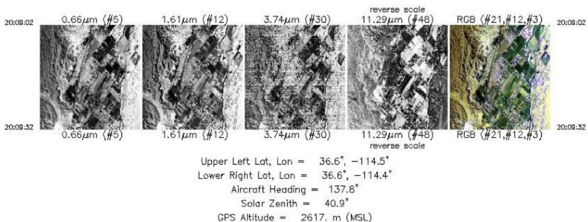
Figure 1. Single-band images and a RGB composite image from flight track 1 acquired on 01 October 2002 near Lake Mead, Nevada, U.S. Source: MASTERL1B_0300101_01_20021001_2009_2009_V01.jpg
