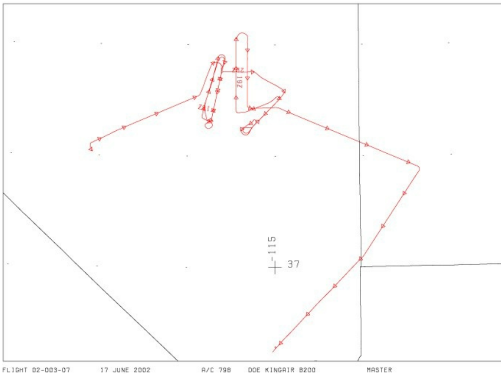
Figure 3. Flight path is shown for 17 June 2002. Flight 0200307 and 8 flight tracks over western Utah and central Nevada. Source: MASTER_0200307_20020617_flightpath.gif
