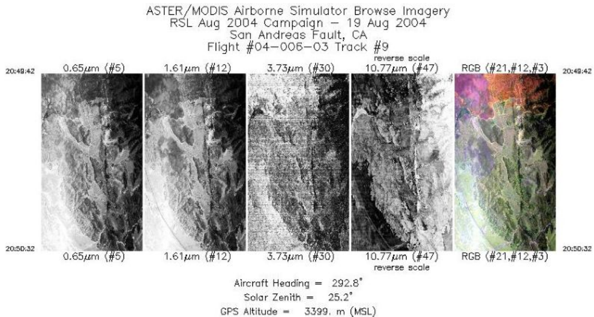
Figure 1. Single-band images and a RGB composite image from flight track 9 acquired on 19 August 2004 over the San Andreas Fault east of Riverside, California, U.S. Source: MASTERL1B_0400603_09_20040819_2049_2050_V01.jpg
