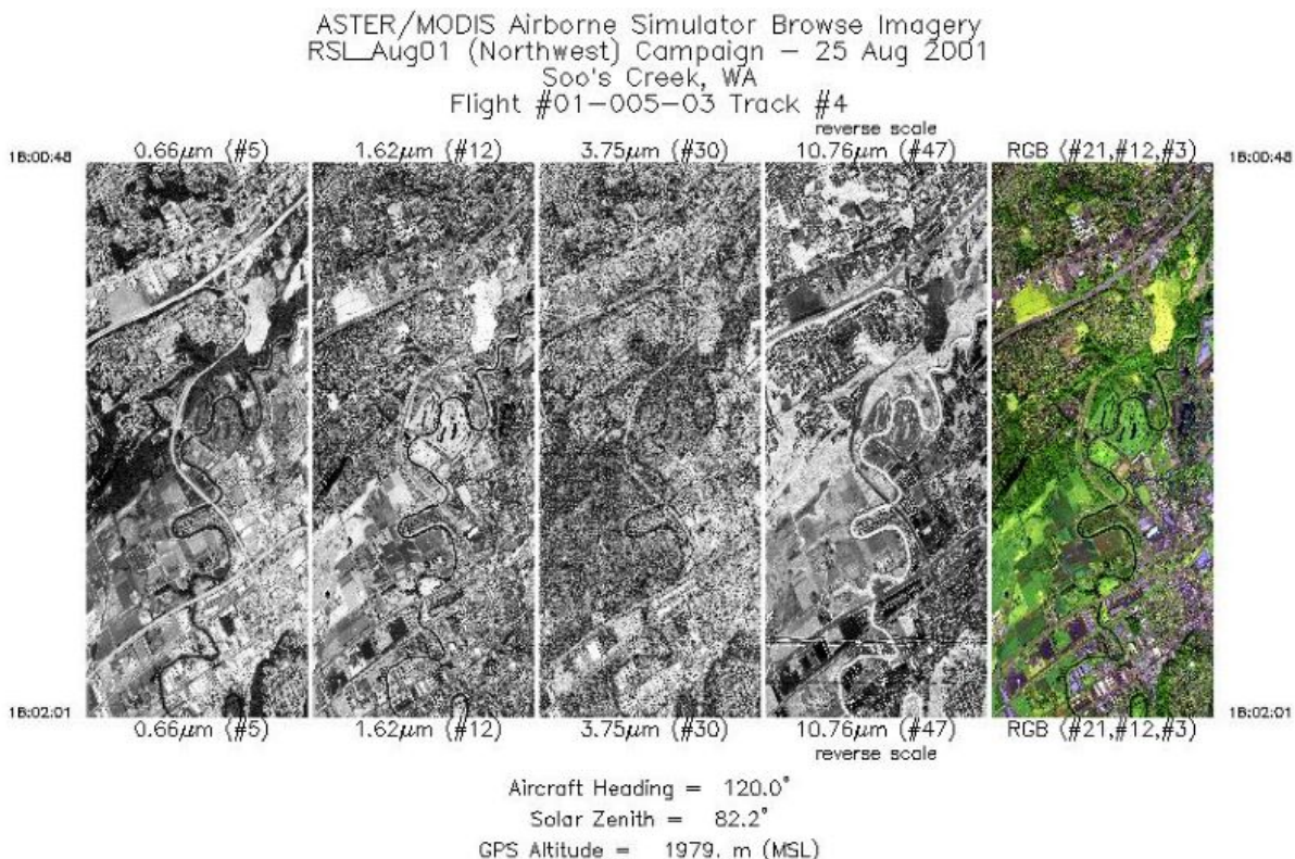
Figure 1. Single-band images and a RGB composite image from flight track 4 acquired on 25 August 2001 over Soo's Creek west of Kent, Washington, U.S. Source: MASTERL1B_0100503_04_20010825_1800_1802_V01.jpg
