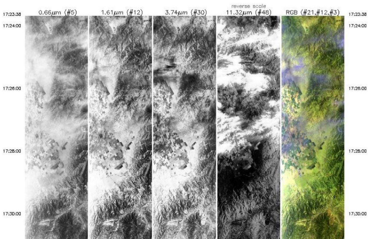
ASTER/MODIS Airborne Simulator Browse Imagery HypsIRI/Late Summer 2014 Campaign - 29 Aug 2014 Santa Barbara Box (Line 10) Flight #14-941-00 Track #3
