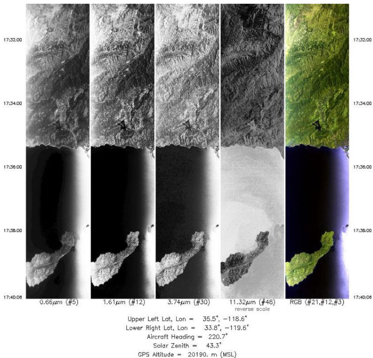
Figure 1. Single band images and an RGB composite image from flight track 3 acquired on 29 August 2014 over the coastal landscape and Santa Cruz Island south of Santa Barbara, California. Source: MASTERL1B_1494100_03_20140829_1723_1740_V01.jpg
