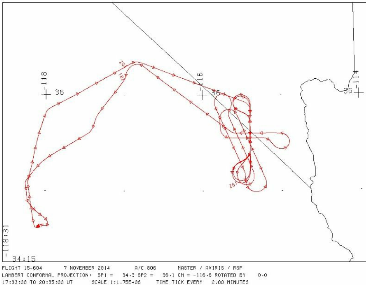
Figure 3. Flight path for Flight 1560400, flown on 07 November 2014. Flight 1560400 and 10 flight tracks occurred over southern California and western Nevada, U.S. Source: MASTER_1560400_20141107_flightpath.gif
