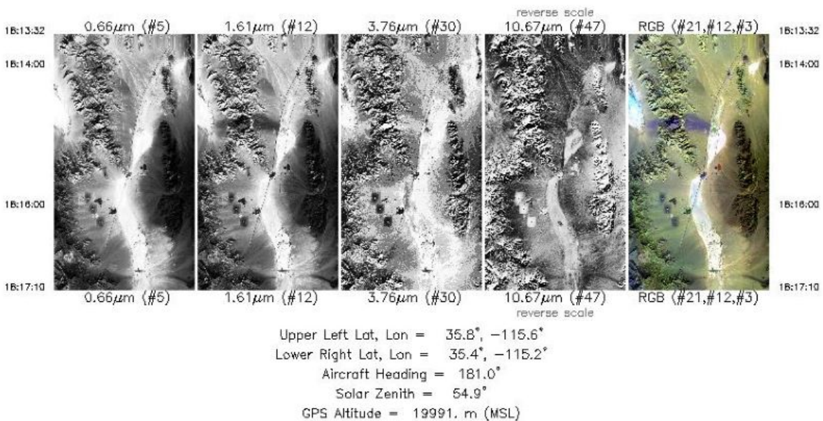
Figure 1. Single band images and an RGB composite image from flight track 1 acquired on 07 November 2014 near Pimm, Nevada, along the California border. Source: MASTERL1B_1560400_01_20141107_1813_1817_V01.jpg
