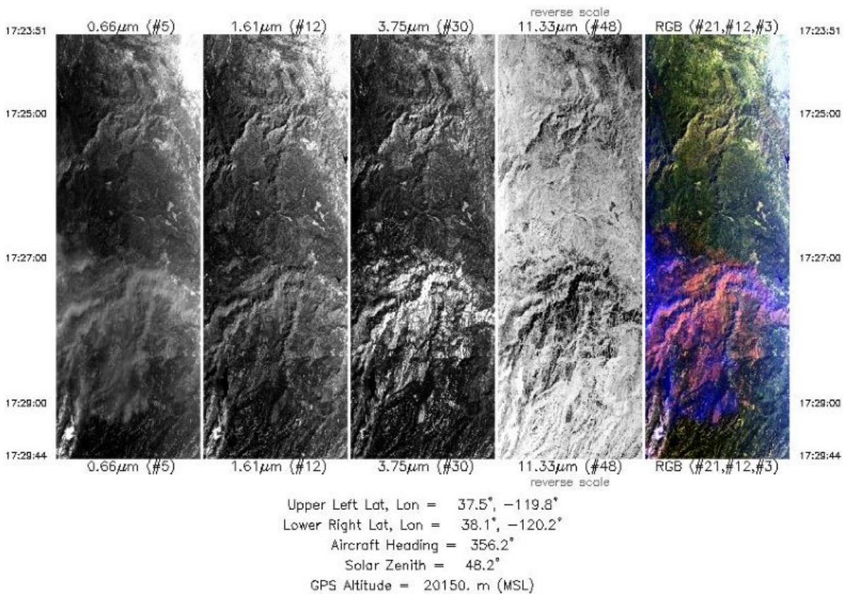
Figure 1. Single band images and an RGB composite image from flight track 1 acquired on 13 September 2013 over the Rim Fire scar at Yosemite National Park, California, U.S. Source: MASTERL1B_1364500_01_20130913_1723_1729_V03.jpg
