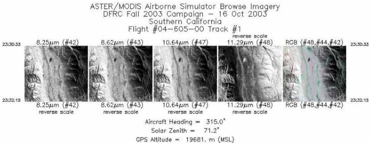
Figure 1. Single-band images and a RGB composite image from flight track 1 as acquired on 16 October 2003 over Lee Vining, California, U.S. Source: MASTERL1B_0460500_01_20031016_2330_2332_V01.jpg
