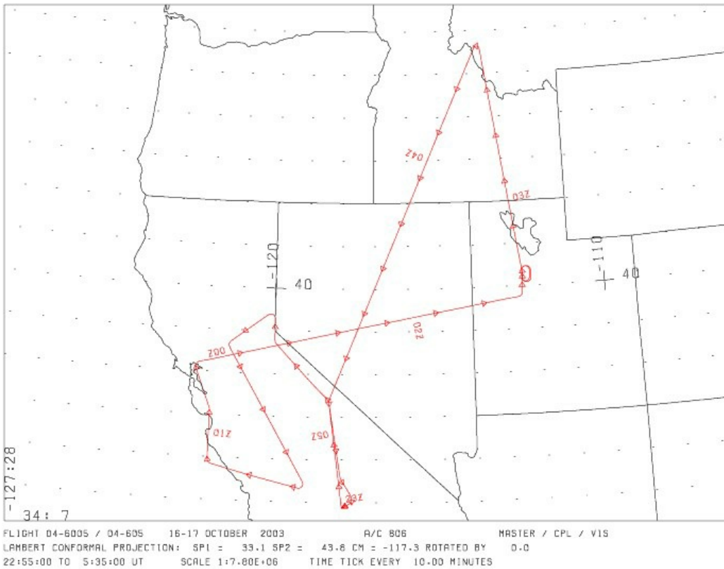
Figure 3. Typical flight path is shown for October 16, 2003 over western US. Flight 0460500 and 19 flight tracks. Source: MASTER_0460500_20031016_flightpath.gif
