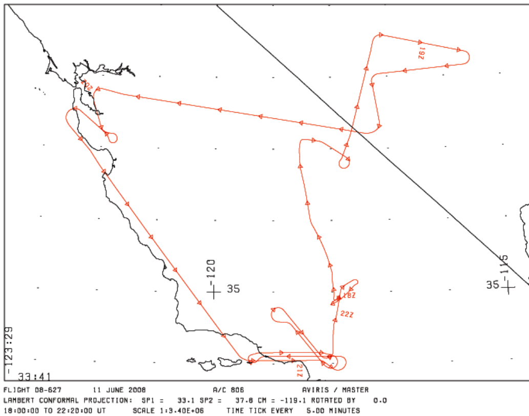
Figure 3. Typical flight path is shown for June 19, 2018. Flight 0862700 and 18 flight tracks. Source MASTER_0862700_20080611_flightpath.gif
