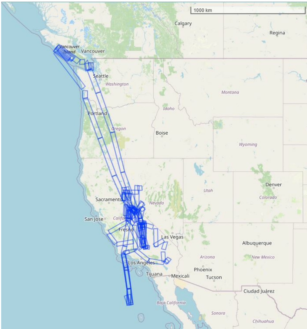
Figure 2. Flight tracks in this dataset represented as blue rectangular polygons. Basemap: © OpenStreetMap contributors.
