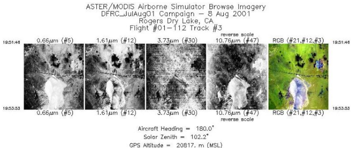
Figure 1. Single-band images and a RGB composite image from flight track 3 as acquired on August 8, 2001 over Rogers Dry Lake northeast of Los Angeles, California, U.S. Source: MASTERL1B_0111200_03_20010808_1951_1953_V01.jpg
