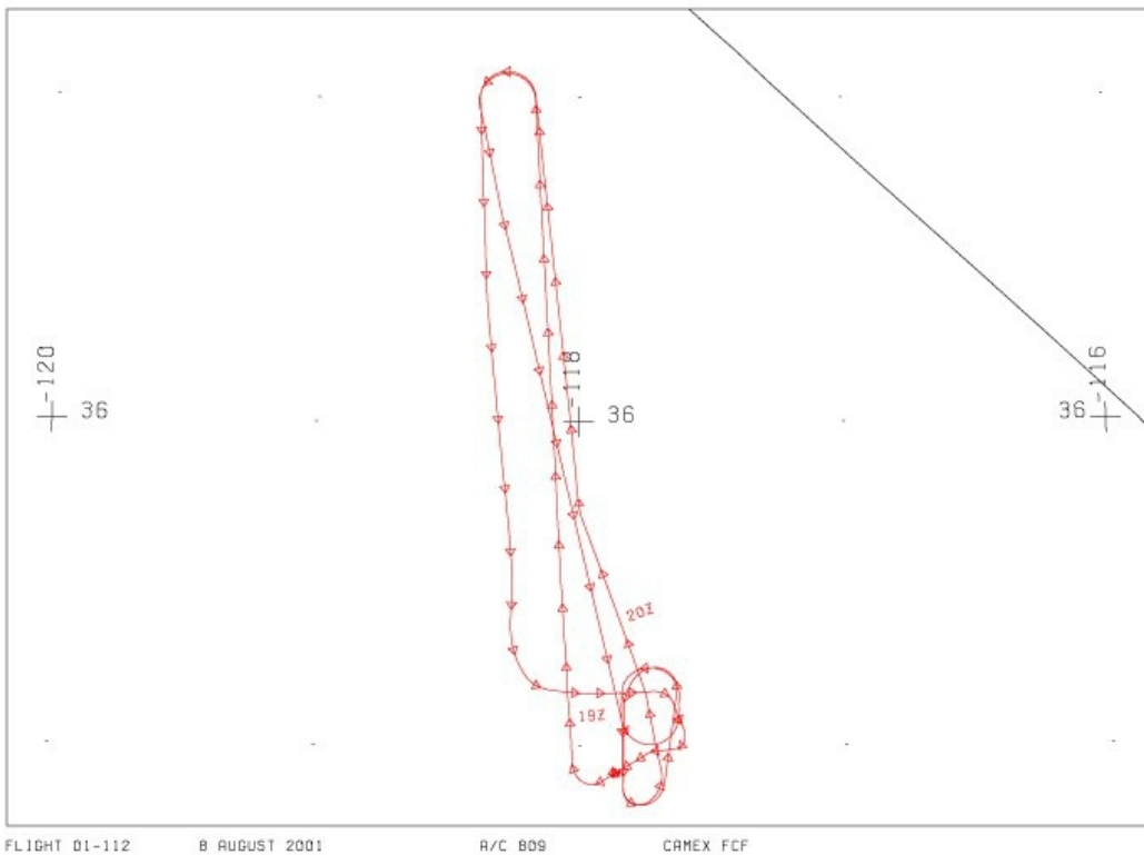
Figure 3. Typical flight path is shown for August 8, 2001 over southern California. Flight 0111200 and 6 flight tracks. Source: MASTER_0111200_20010808_flightpath.gif
