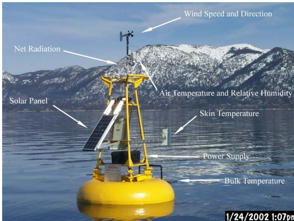
Figure 21: Raft Measurements.
