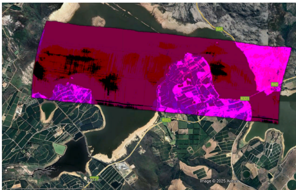
Figure 1. Overlay of L1 radiance data from NASA's Hyperspectral Thermal Emission Spectrometer (HyTES) instrument acquired on November 15 2023. RGB composite bands: 150 (10.1 microns), 100 (9.2 microns), and 58 (8.5 microns). This scene is located west of Theewaterskloof, Western Cape province, South Africa (approximately -34.02 latitude, 19.17 longitude). Background image from Google Earth and Airbus. Source: 20231115t124818_TheewatersBox19ZA_L1_B110_V03.kmz
