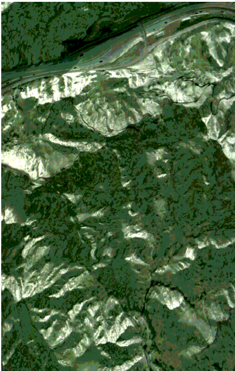
Figure 1. Portion of a false color image derived from HyTES radiance data from flight over Aliso Canyon east of Rancho Mission Viejo, California. Flight 2016-01-26.233621.
