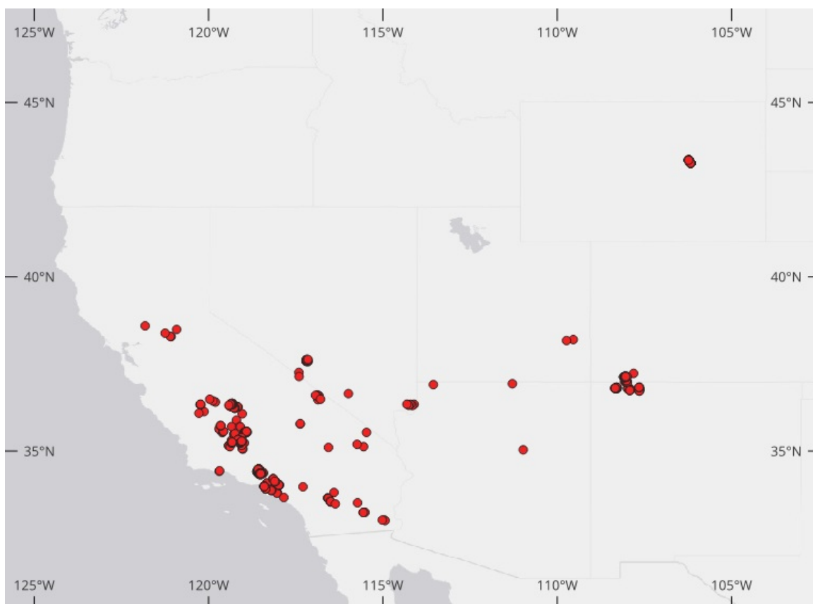
Figure 3. Locations of HyTES flights in 2013 to 2016.
