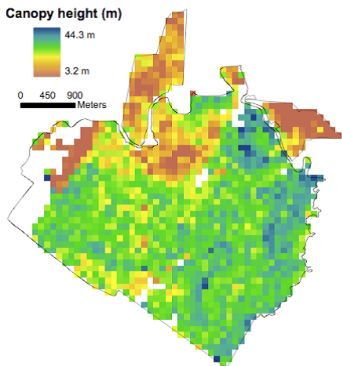
Figure 1. Lidar-derived mean vegetation canopy height in 1998 at 100-m (1-ha) resolution at La Selva Biological Station in Costa Rica (from ls98_ht.tif).
