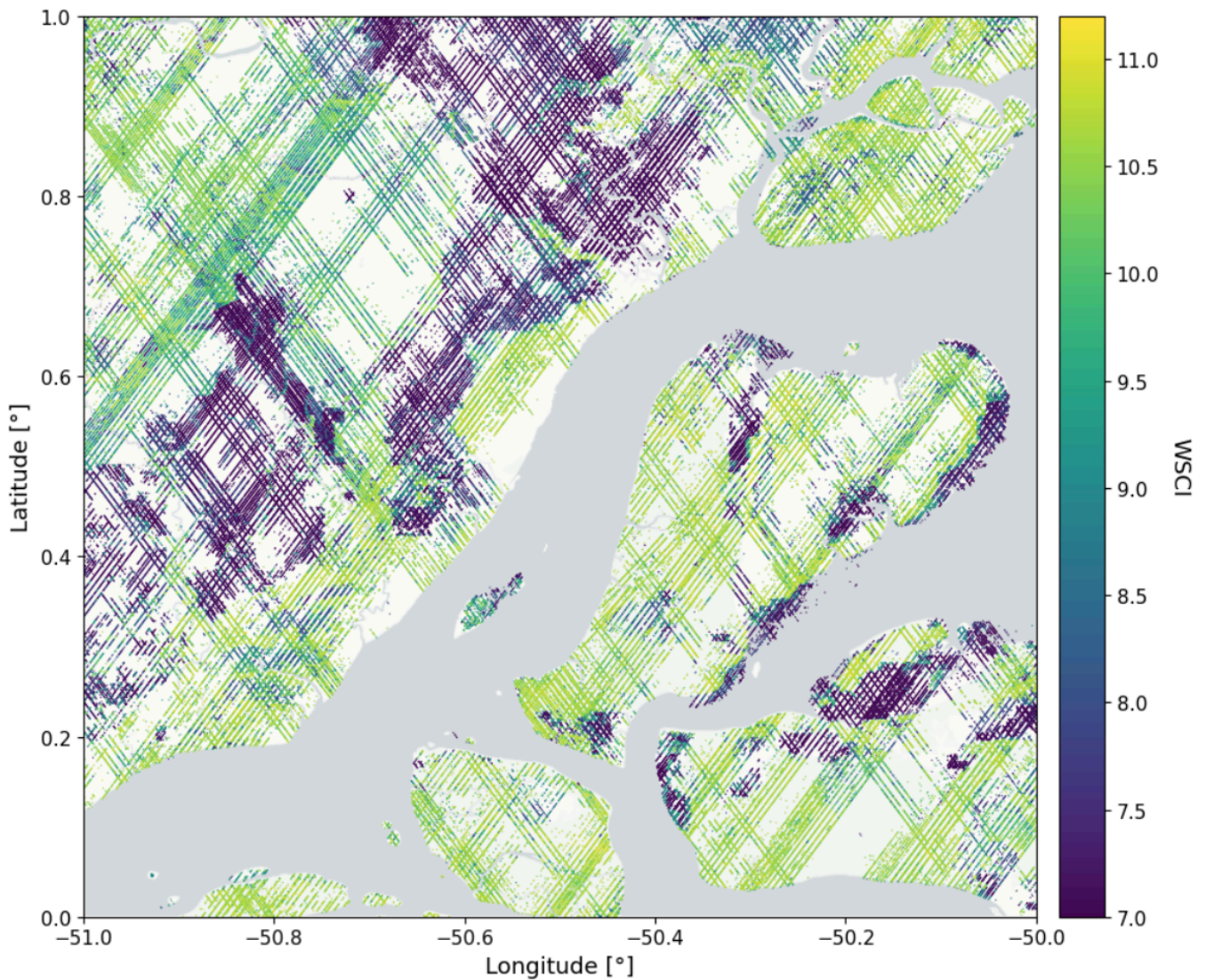
Figure 1. Example subset of the Waveform Structural Complexity Index (WSCl) predictions from the GEDI Level-4C footprint product over the eastern Amazon.
