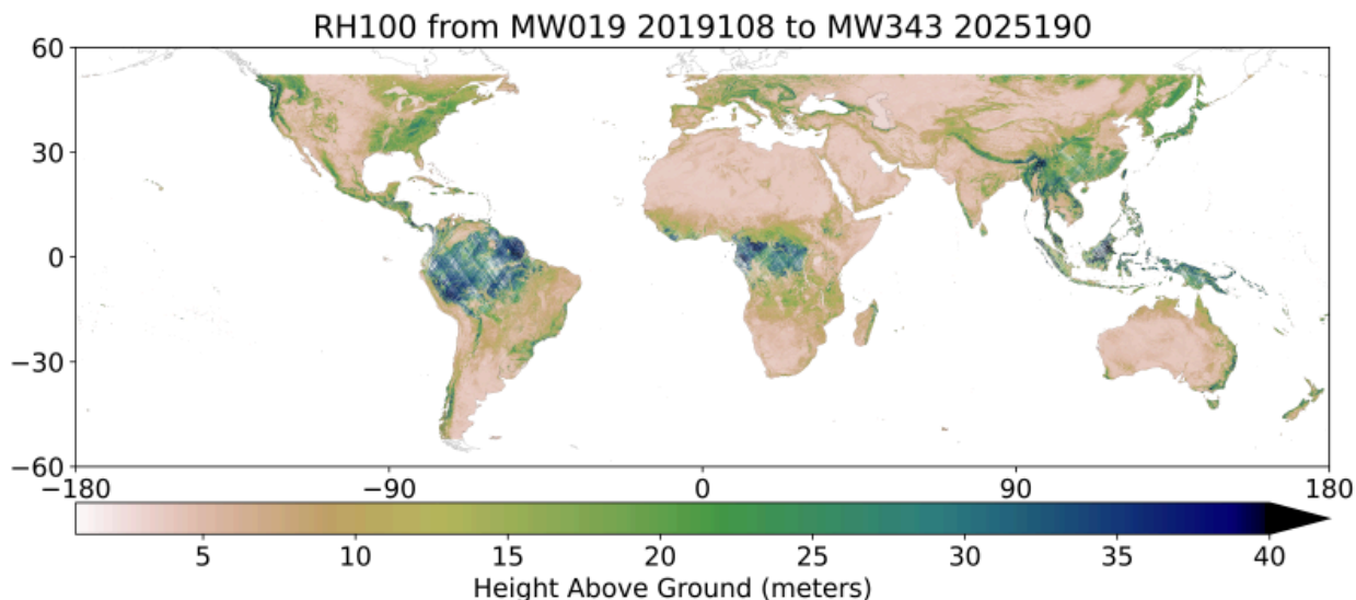
Figure 1. Level 3 estimated canopy height in meters derived from the GEDI Level 2 profile metric RH100 between the 19th and the 343rd mission week. Source: GEDI03_rh100_mean_2019108_2025190_003_01.tif
