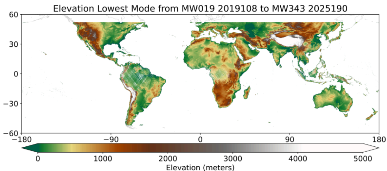
Figure 3. Estimated mean elevation of lowest mode. Image derived from the dataset file GEDI03_elev_lowestmode_mean_2019108_2025190_003_01.tif.
