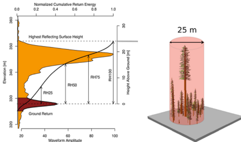
Figure 2. Sample of the GEDI lidar waveform (left). The light brown area under the curve represents return energy from the canopy, while the dark brown area signifies the return from the underlying topography. The black line is the cumulative return energy, starting from the bottom of the ground return (normalized to 0) to the top of the canopy (normalized to 1). RH metrics give the height at which a certain quantile returned energy is reached relative to the ground (i.e., the center of the ground return). The diagram on the right shows the distribution of trees that produced the waveform.
