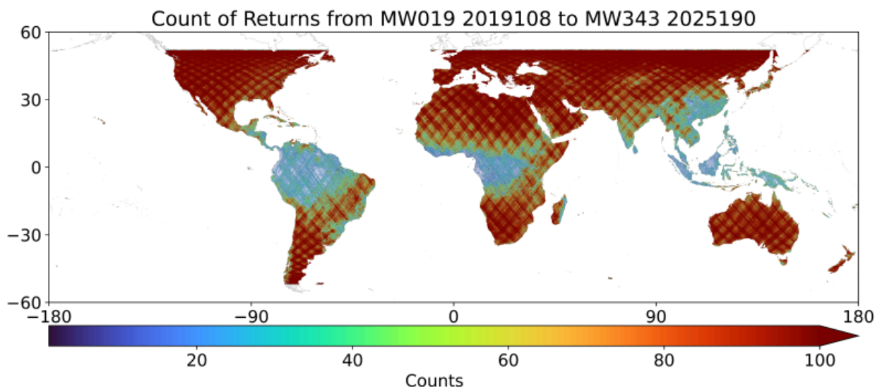
Figure 5. Count of valid laser footprints per grid cell. Image derived from dataset file GEDI03_counts_2019108_2025190_003_01.tif.
