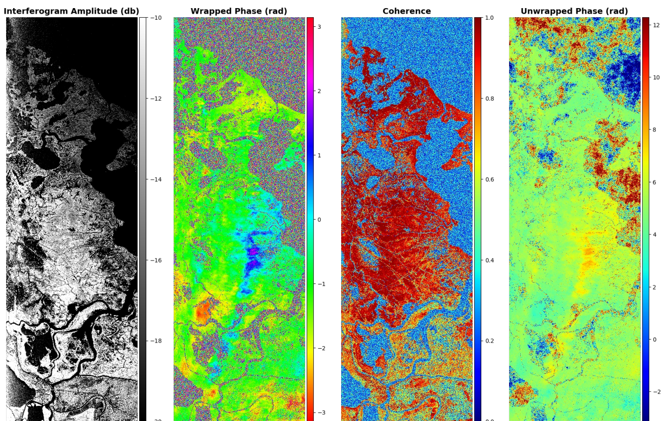
Figure 1. UAVSAR interferometric product example. From left to right: Interferometric amplitude (displayed in decibel scale), wrapped interferometric
