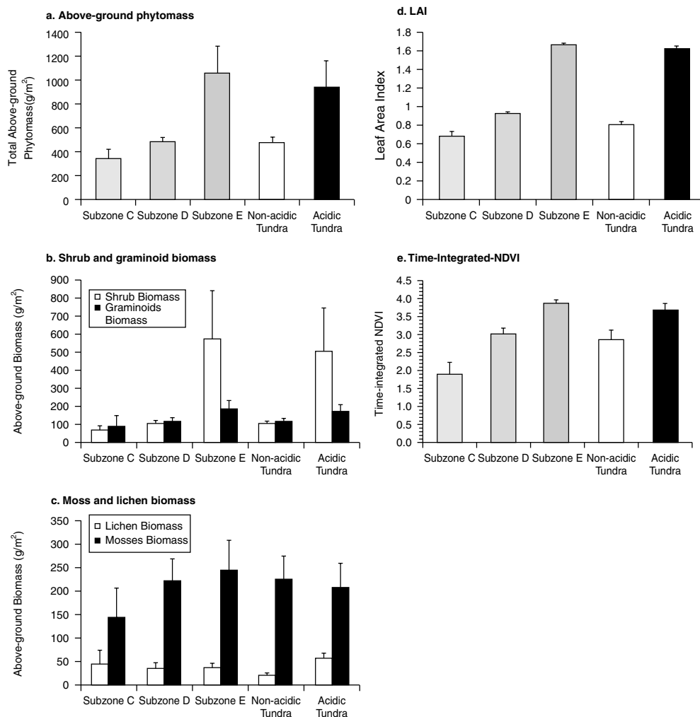
Figure 6 Summary of means ( \pm standard errors) for key biological variables by bioclimate subzones and soil reaction class: (a) above-ground phytomass, (b) shrub and graminoid phytomass, (c) moss and lichen phytomass, (d) LAI, and (e) total Integrated NDVI.
