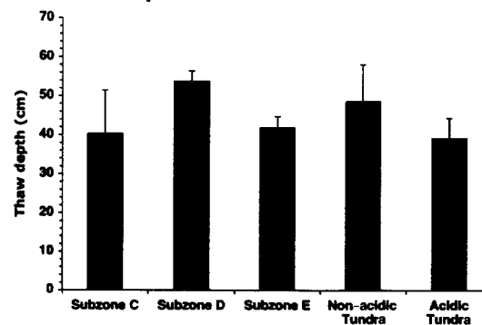
Figure 4 Summary of means ( \pm standard errors) for three key physical variables by bioclimate subzone and acidic and non-acidic tundra: (a) SWI, (b) soil organic horizon thickness, and (c) late-August thaw depth.
