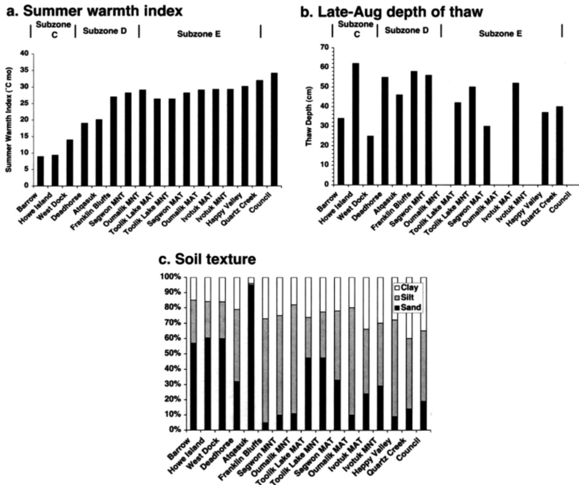
Figure 3 Comparison of physical variables for the study sites arranged by subzone. (a) SWI, (b) late-August depth of thaw, and (c) soil texture. Gaps in (b) are due to either missing data (Oumalik MNT and MAT), or rocky soils (Ivotuk MNT), or have no permafrost (Council).
